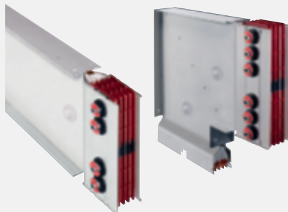
2 SOLUTION FOR THE DISTRIBUTION OF HIGH CURRENTS
