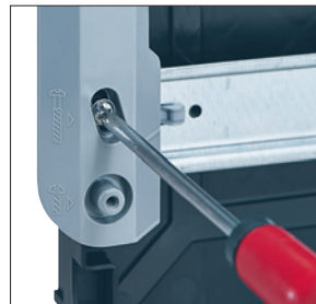
2 REMOVABLE FRAME Allows wiring in the workshop. Vertical level adjustment possible thanks to the oblong holes.
